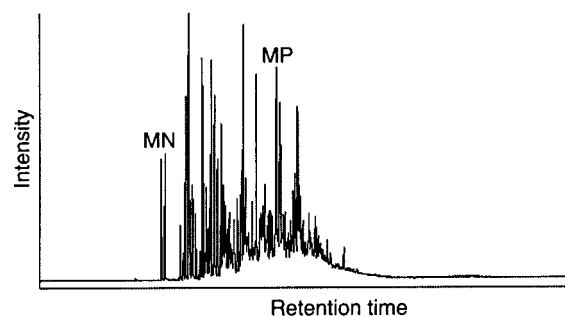
Fig. 2 Partial total ion chromatogram obtained during GC-MS (selected ion monitoring) analysis of the aromatic hydrocarbons isolated from diesel. Key: MN = methyl-naphthalenes, MP = methyl-phenanthrenes.
